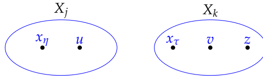
Figure 5: Points in Proof of Lemma 4
